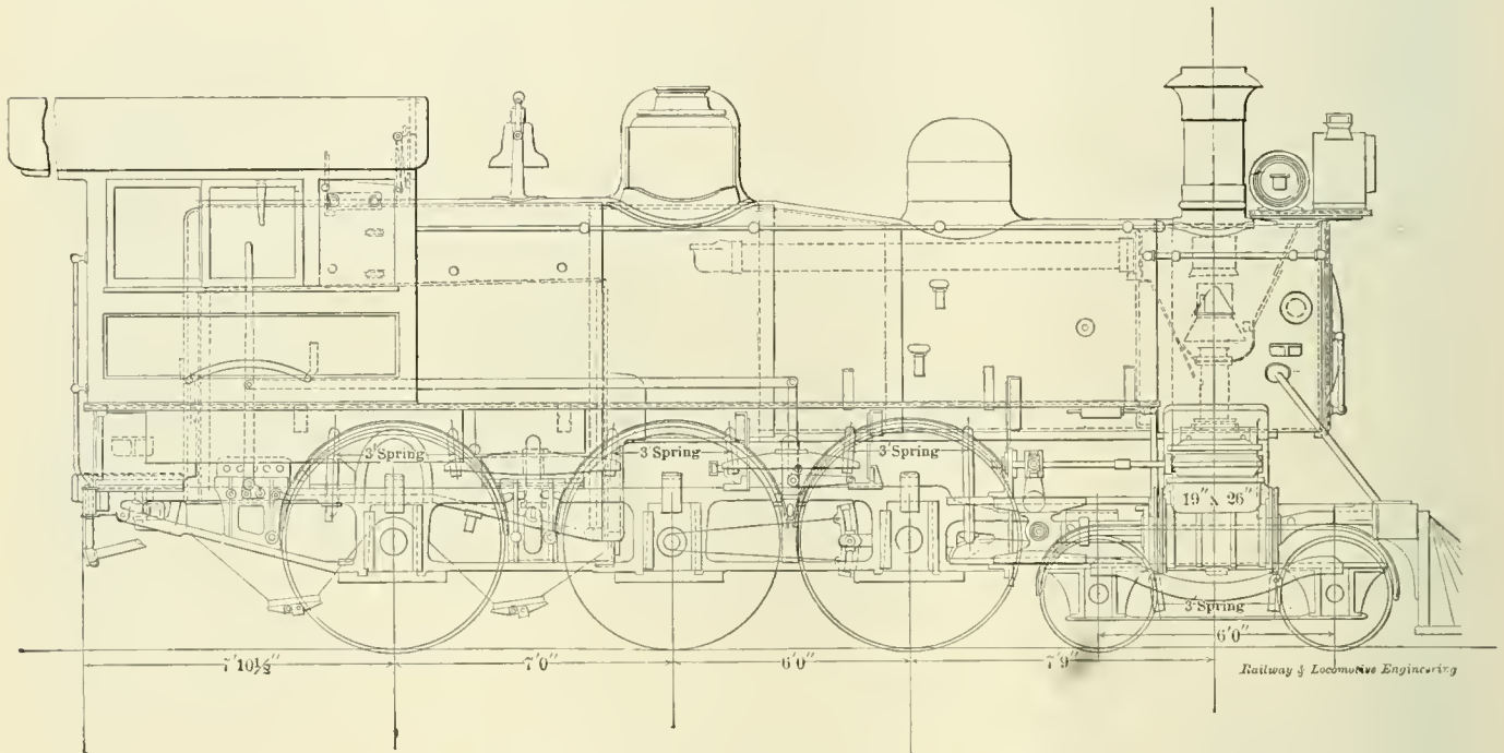
ROGERS TEN-WHEEL ENGINE FOR THE N., C. & ST. L.
